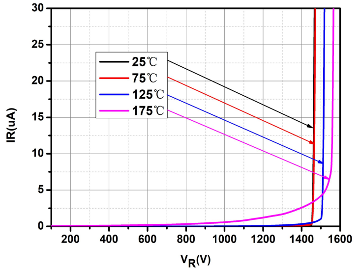
Fig.2-Typical Reverse Characteristics
